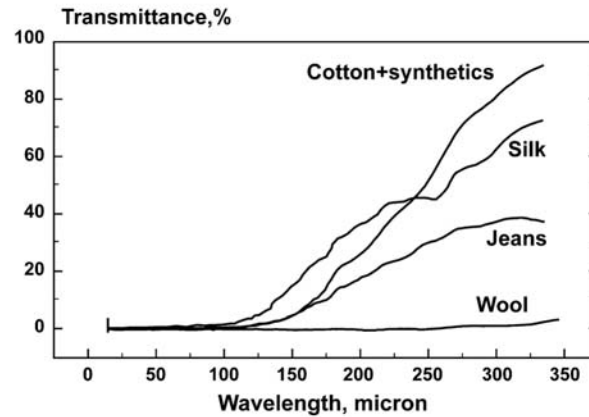
Fig. 9 Transmittance of different clothes versus wavelength.
